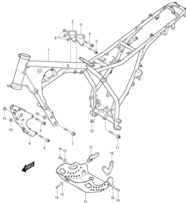
FIG27Rahmen
