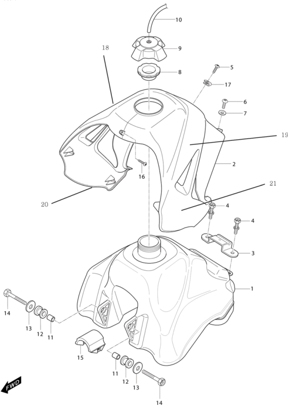
FIG30Tank
